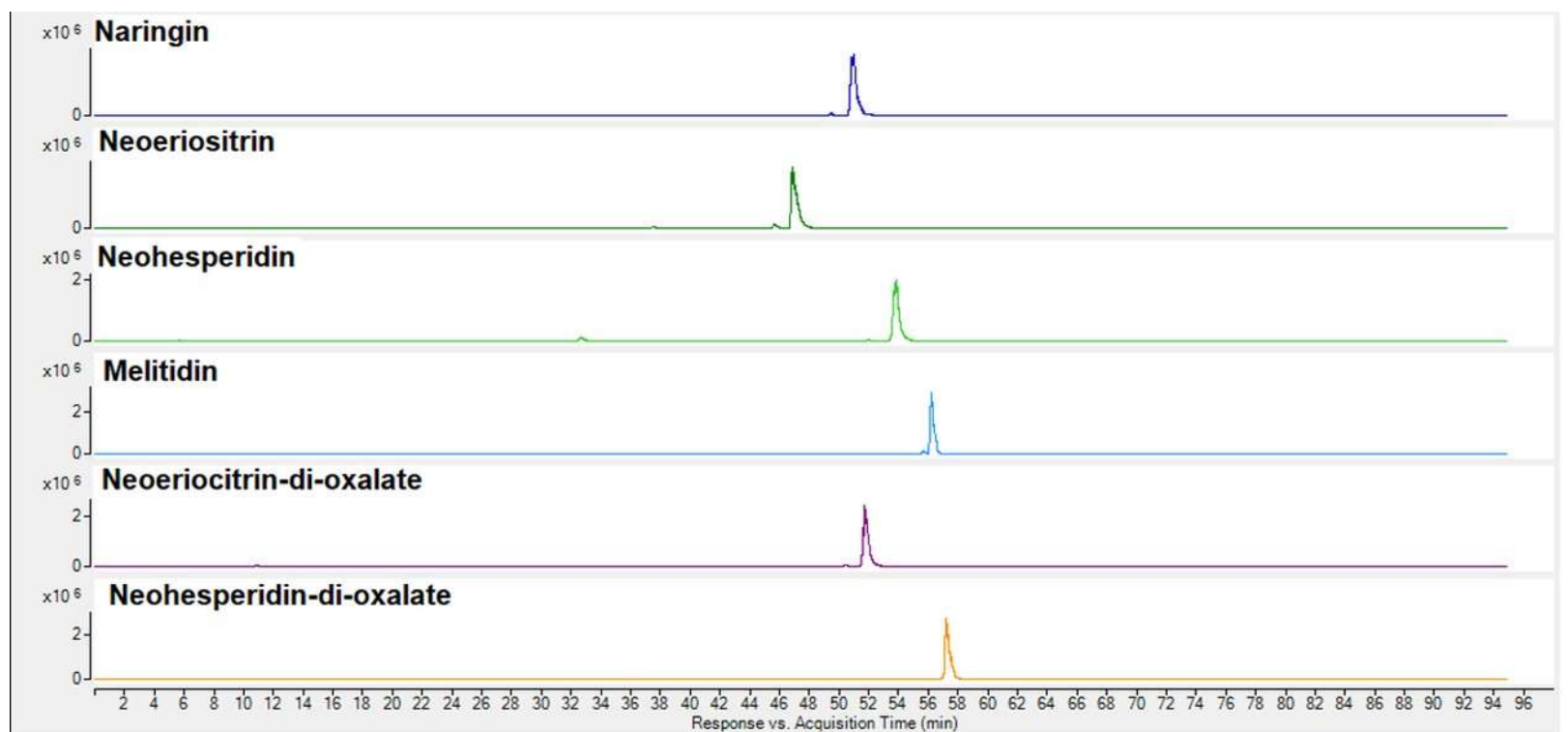
Figure S1. LC-ESI-MS/MS chromatograms of phenolic compounds identified in the supernatant from bergamot fruit homogenate.
