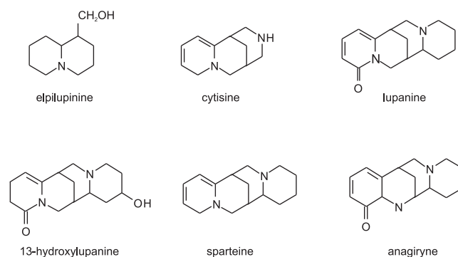
FIGURE 2. Structures of lupine alkaloids [Gulewicz, 1988].
