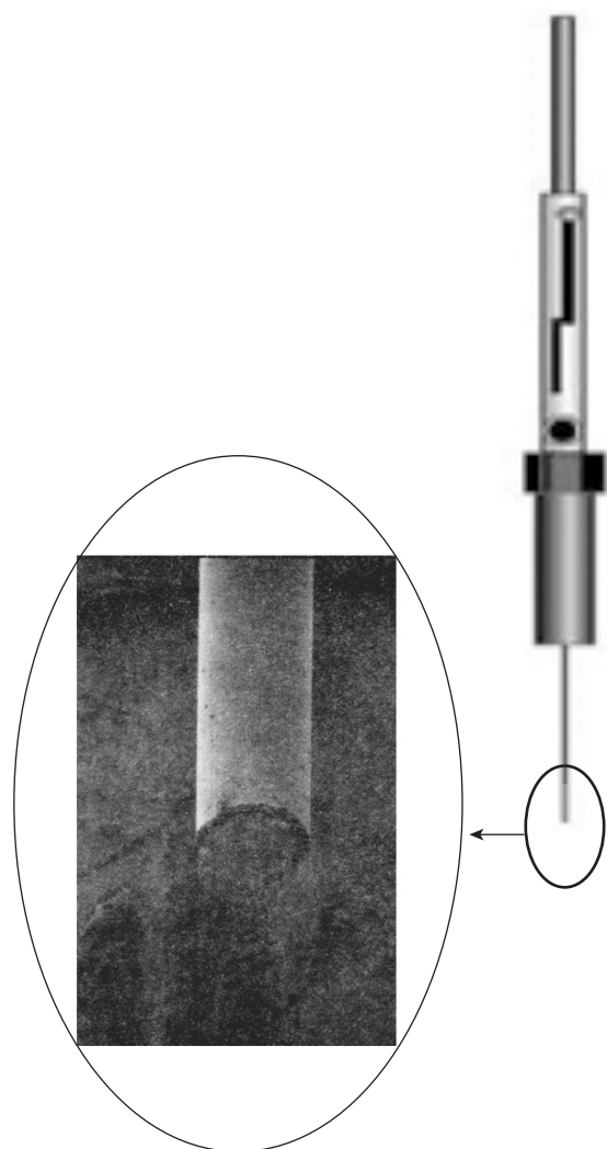
FIGURE 1. SPME apparatus offered by Supelco Inc. with the picture of a scanning electron micrograph of polymer-coated film of SPME fiber.
