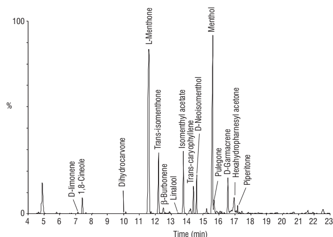
FIGURE 6. GC/MS chromatogram of volatile organic compounds obtained from Mentha piperita extract.
