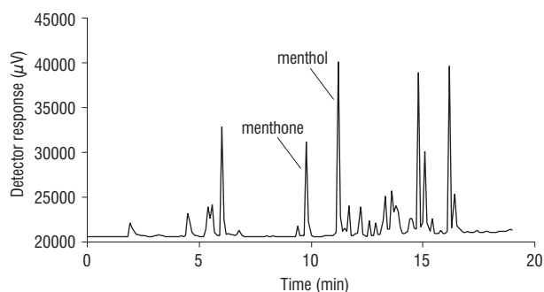
FIGURE 5. Typical chromatogram obtained from peppermint candy sample after the use of ca. 10 \mu\text{m} PDES-coated fiber.
