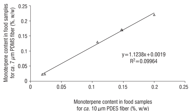
FIGURE 3. The correlation of monoterpenes concentrations in food samples isolated using various SPME fibers.
