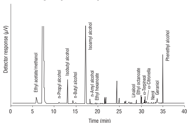
FIGURE 4. SPME-GC chromatogram of a red wine sample.
