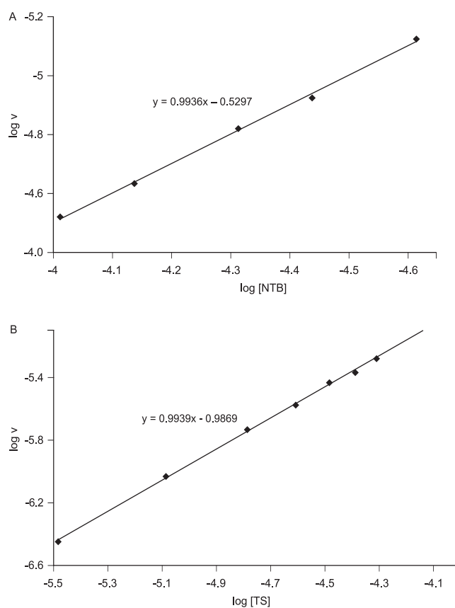
FIGURE 5. Determination of the order of reaction between NTB and garlic thiosulfinates using the initial rate method.
