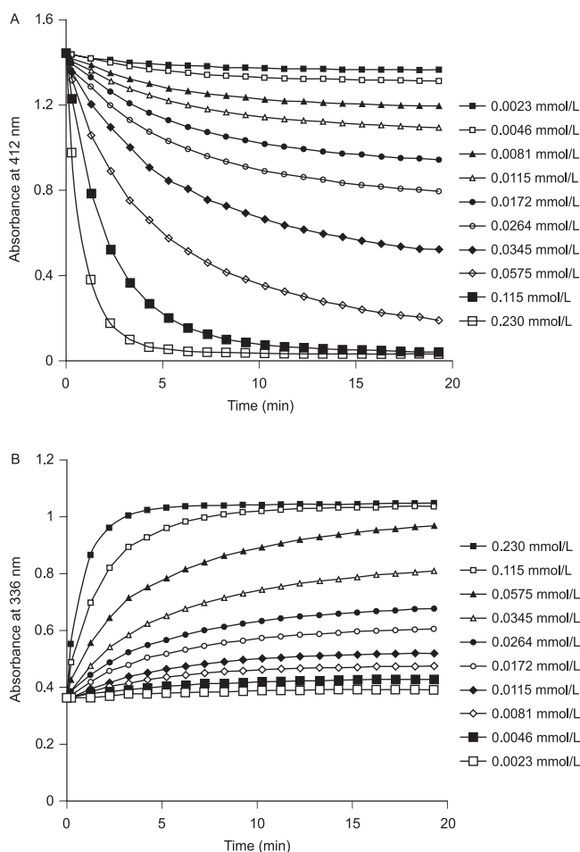
FIGURE 4. Kinetics of the reaction between 102 \mu\text{mol/L} solution of 2-nitro-5-thiobenzoic acid and garlic thiosulfinates. Concentrations of TS are given in the figures. The reaction course monitored at 412 nm (A) and 336 nm (B).
