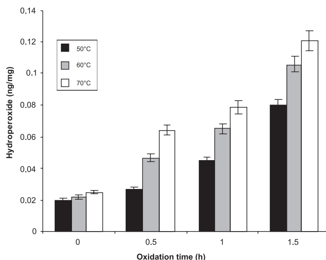
FIGURE 3. Hydroperoxides formation during thermal oxidation of PC membrane at 50°C, 60°C and 70°C measured after 0, 30, 60 and 90 min of oxidation.
