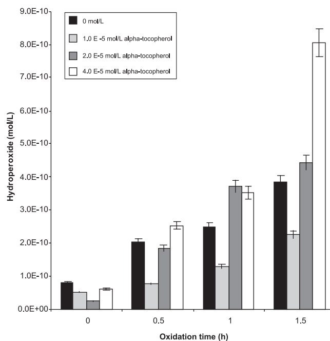
FIGURE 4. The amount of hydroperoxides measured in the presence of 0, 1 \times 10^{-5} , 2 \times 10^{-5} and 4 \times 10^{-5} mol/L of alpha-tocopherol during oxidation of 2 mg/mL PC at 50°C.
