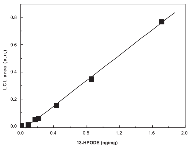
FIGURE 2. Calibration curve obtained as a plot of integrated LCL signal versus standard 13-HPODE concentration. The other concentrations of mixture as given in the Legend to Figure 1.
